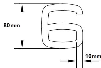
Picture 21 – Prototype rear number minimum dimensions
