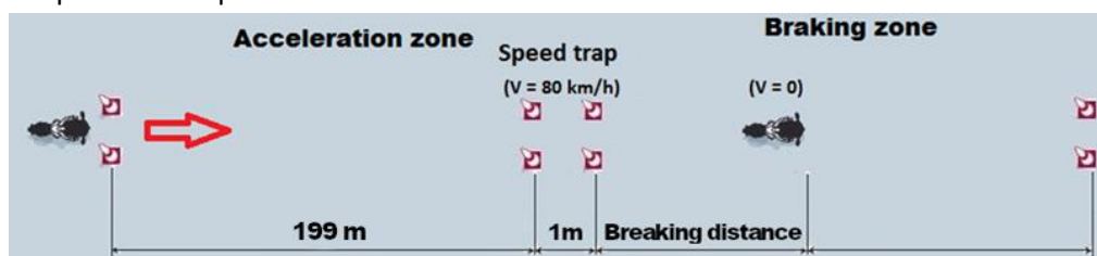
Picture 45 - Graphic description of MS1 Test 1: Brake
