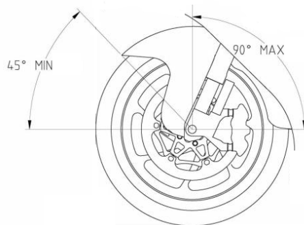
Picture 13 - Prototype front mudguard
